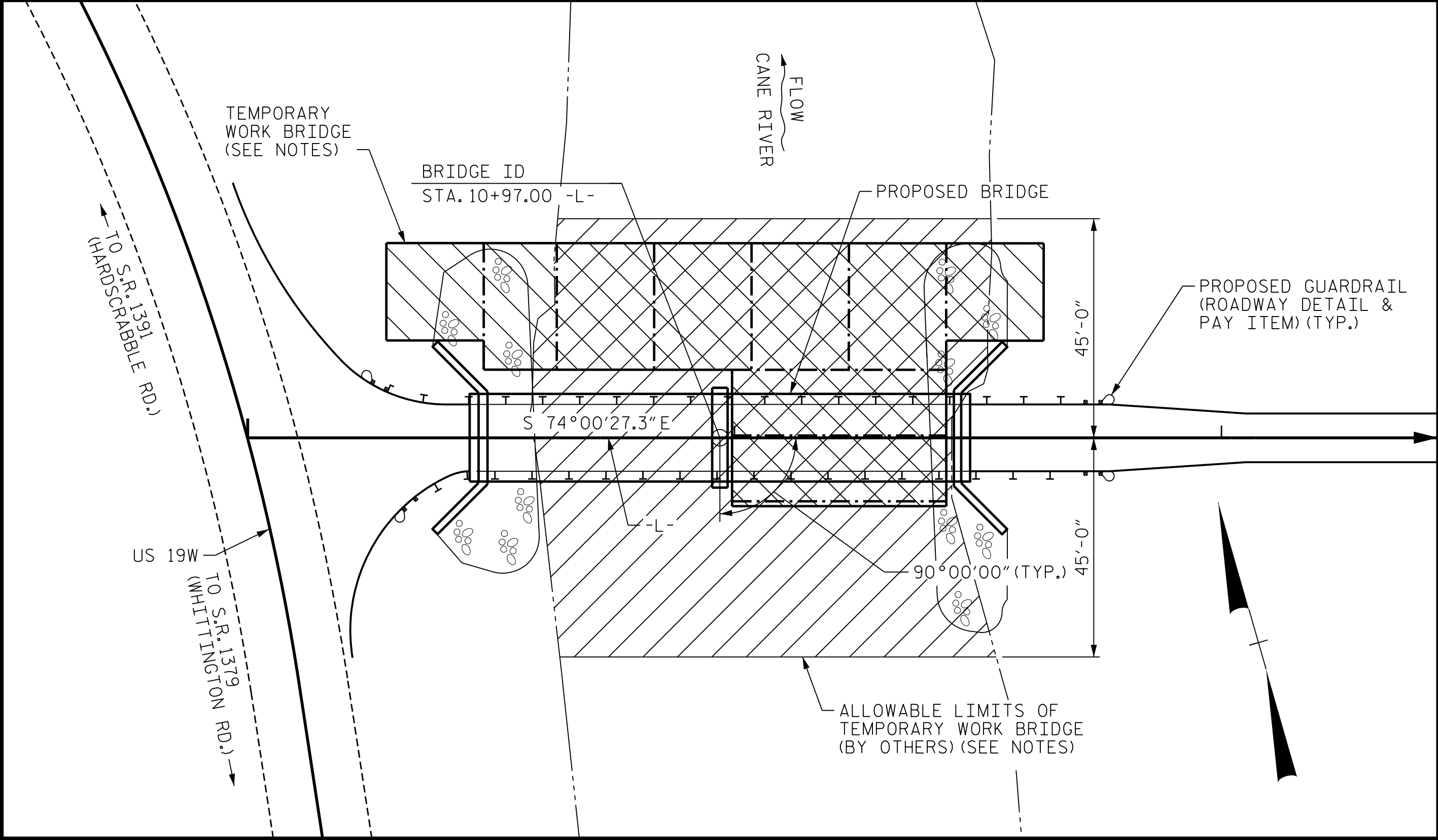
LOCATION SKETCH
