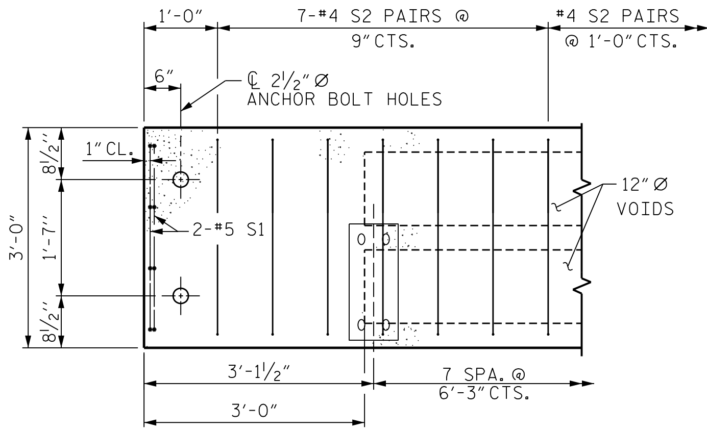
DETAIL "A" (TYPICAL EACH END OF UNIT) NOTE: EXTERIOR UNIT SHOWN - INTERIOR UNIT SIMILAR
