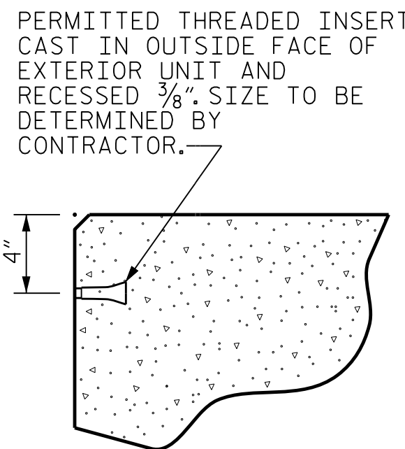
THREADED INSERT DETAIL
