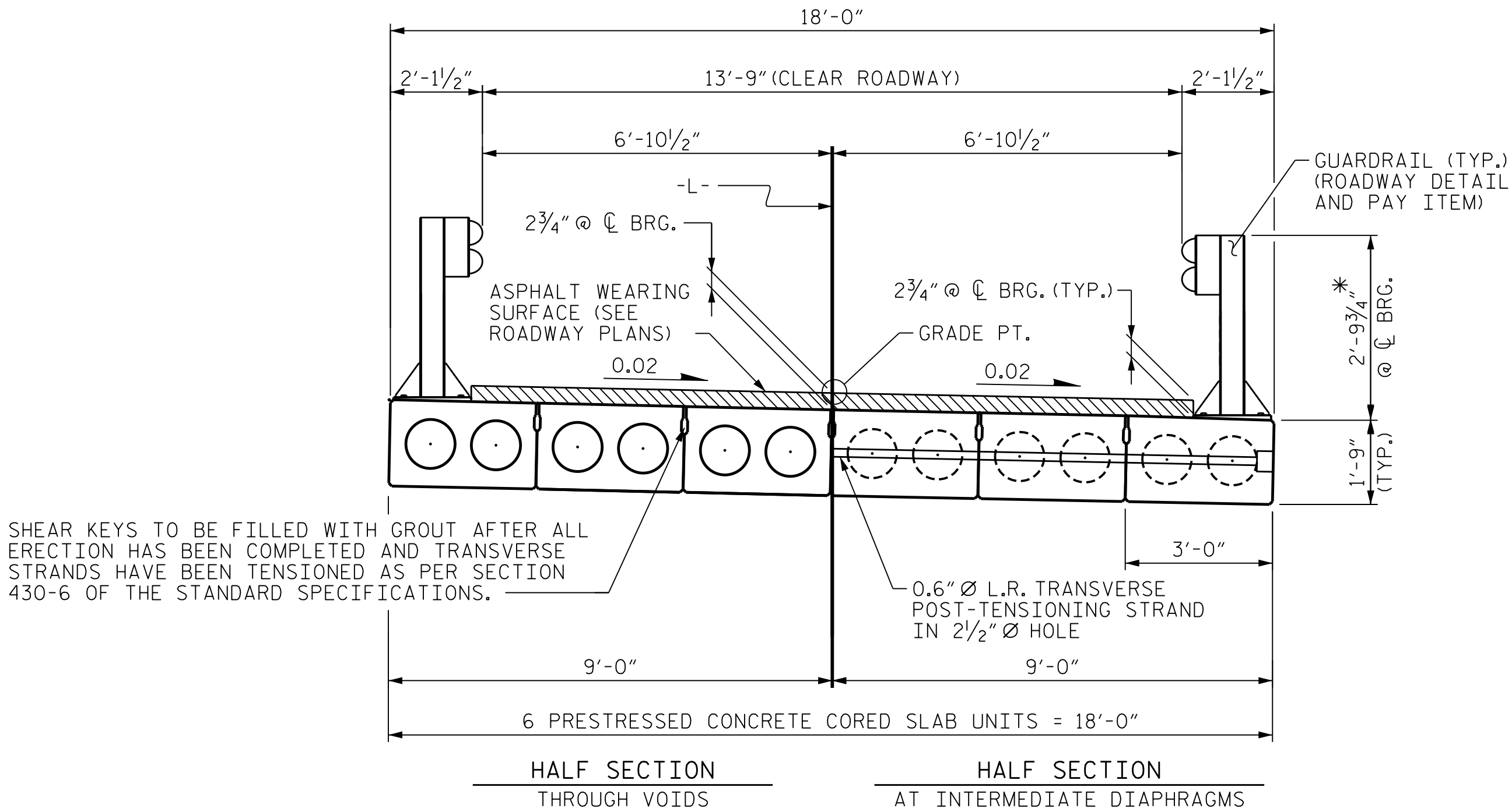
TYPICAL SECTION
