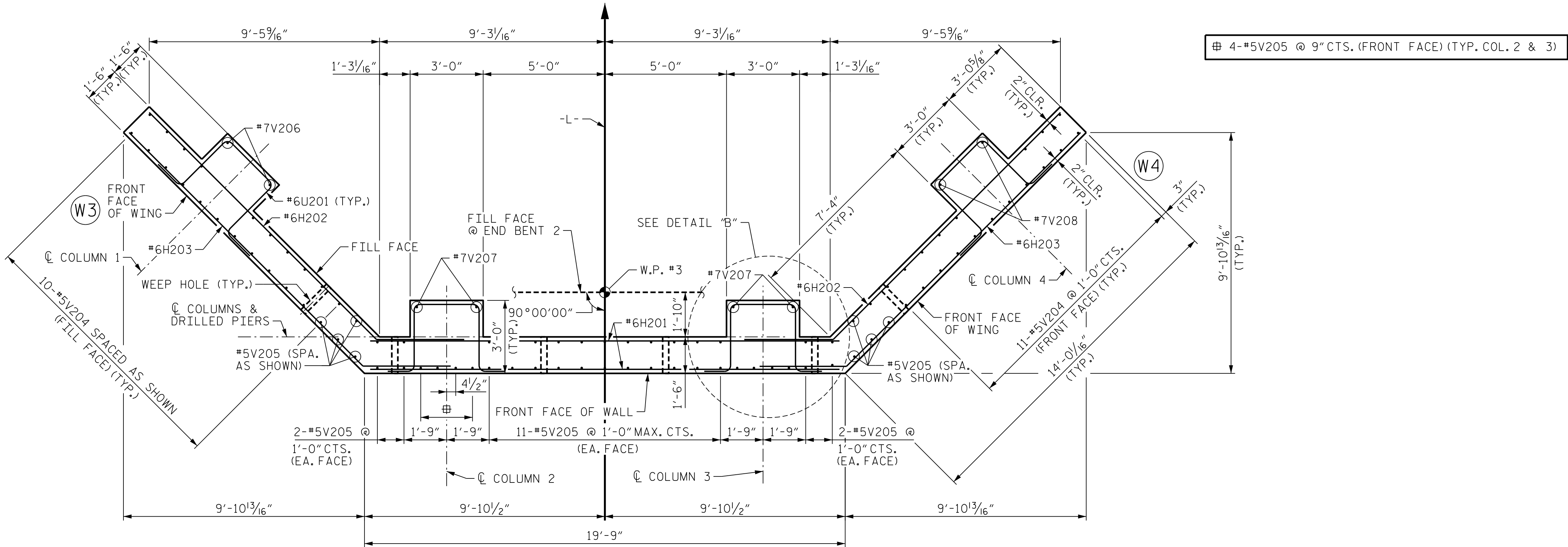
PLAN OF RETAINING WALL (DRILLED PIERS AND MAIN REINFORCEMENT FOR DRILLED PIERS AND COLUMNS NOT SHOWN FOR CLARITY)
