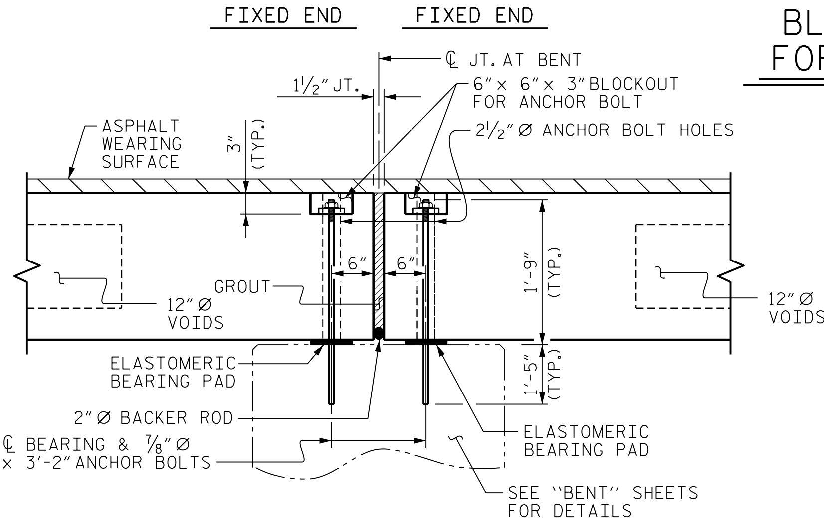
SECTION AT BENT
