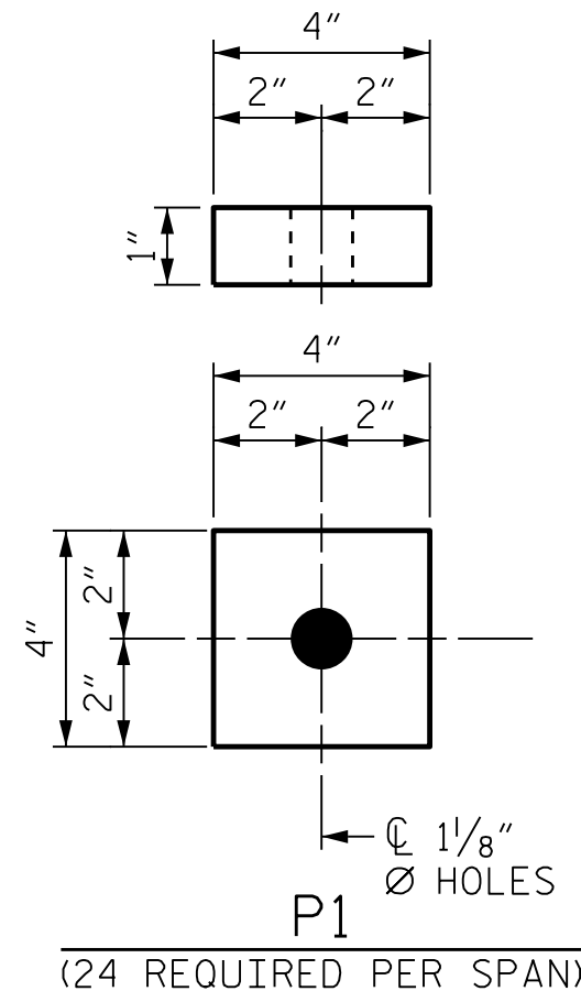
PLATE DETAILS
